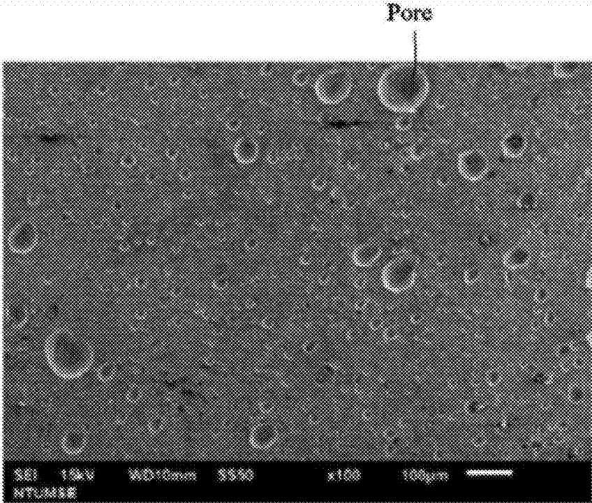
Sapphire + Cu with 50nm Ni-P
