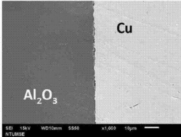
Sapphire + Cu with 50nm Ni-P
